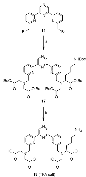
Scheme 2 Reagents and conditions: a) secondary amine 16 (1.1 equiv.), NaI (0.6 equiv.), K 2 CO 3 (15 equiv.), DMF, rt, 9 h then secondary amine 9 (1.05 equiv.), rt, 72 h, 18%; b) TFA, H 2 O (40 equiv.), CH 2 Cl 2 , 0 °C to rt, 20 h, 54%.
